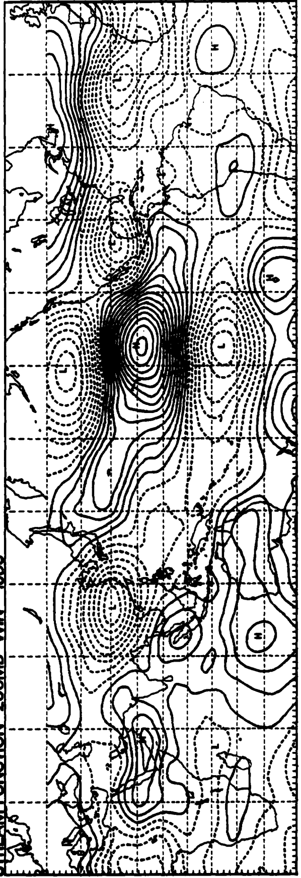
STREAM FUNCTION 200MB WIN 1983
